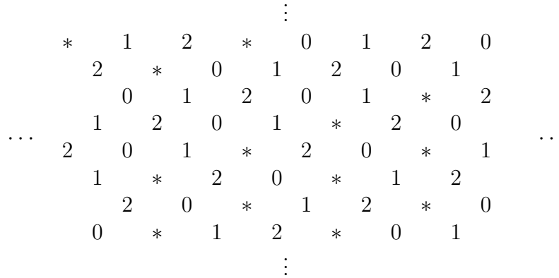
Figure 2: A triangular tiling
