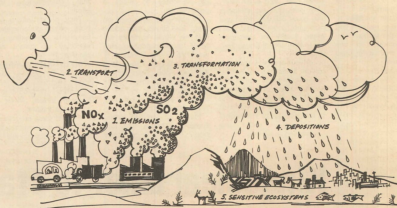
WINDS CARRY POLLUTANTS OVER LONG DISTANCES... HUNDREDS, OR EVEN THOUSANDS OF KILOMETRES
